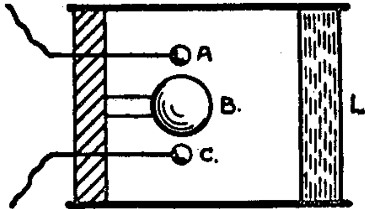
Figure 3 Bose's diagrams of his radiators. (a) shows the radiator used to generated 5-mm radiation, while (b) shows the arrangement with a lens L at the exit of the waveguide [2]. In some designs the mounting stems for the outer spheres could be inclined to adjust the dimension of the spark gaps.
